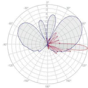
60 ° Service Beam
